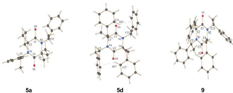
Fig. 2 X-ray crystal structures of 5(a, d) and 9 . Configurations of the stereogenic carbons (in the three structures): C(2) ( S ); C(4) ( S ); C(5) ( S ); C(13) ( S ). C(2) and C(4) atoms correspond to C(3) and C(6) atoms in Scheme 1
