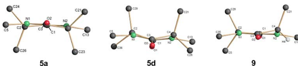
Fig. 4 Conformations of diketopiperazine rings in 5(a, d) and 9
