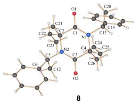
Fig. 5 Molecular structure of 8 . Configurations of the stereogenic carbons are: C(2) ( S ), C(4) ( R ), C(5) ( S ), C(13) ( S )
